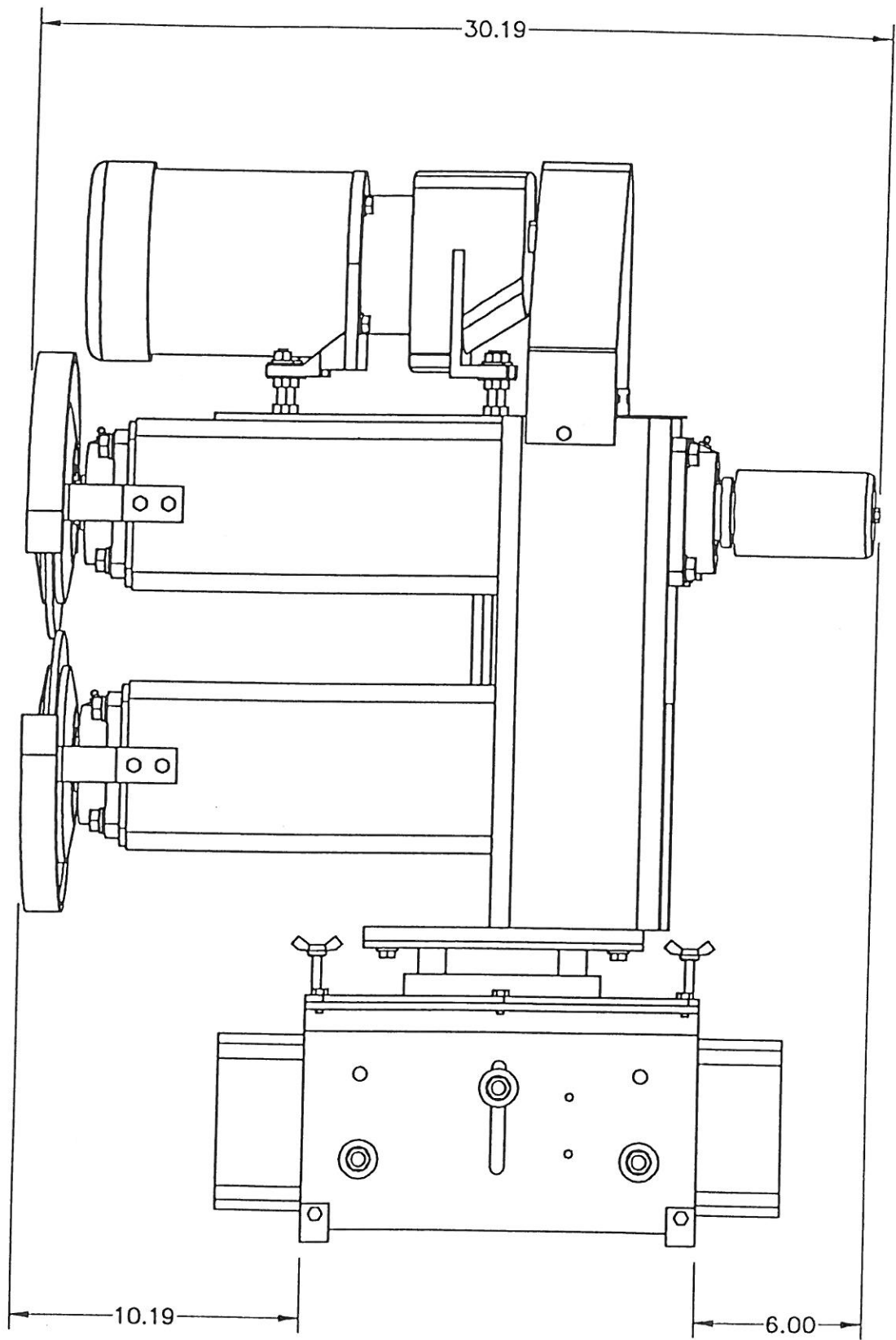
610 LEFT HAND TRIMMER ON A 6" RIGID TROLLEY WITH THE SAME CUT LINE AS A 601 ON A 6" SHORT BLOCK SWIVEL TROLLEY
