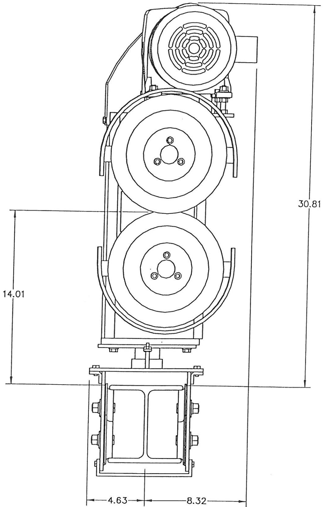
610 RIGHT HAND TRIMMER ON A 6" RIGID TROLLEY WITH THE SAME CUT LINE AS A 601 ON A 6" SHORT BLOCK SWIVEL TROLLEY
